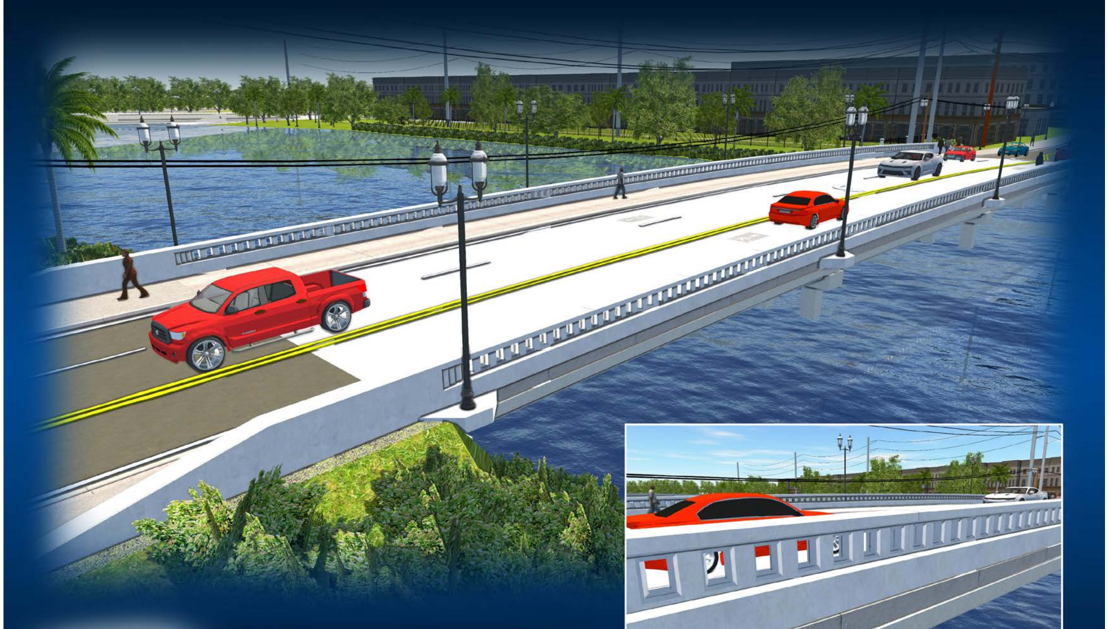
TRAFFIC RAILING BARRIER TYPE C412 TXDOT - 42 INCHES
